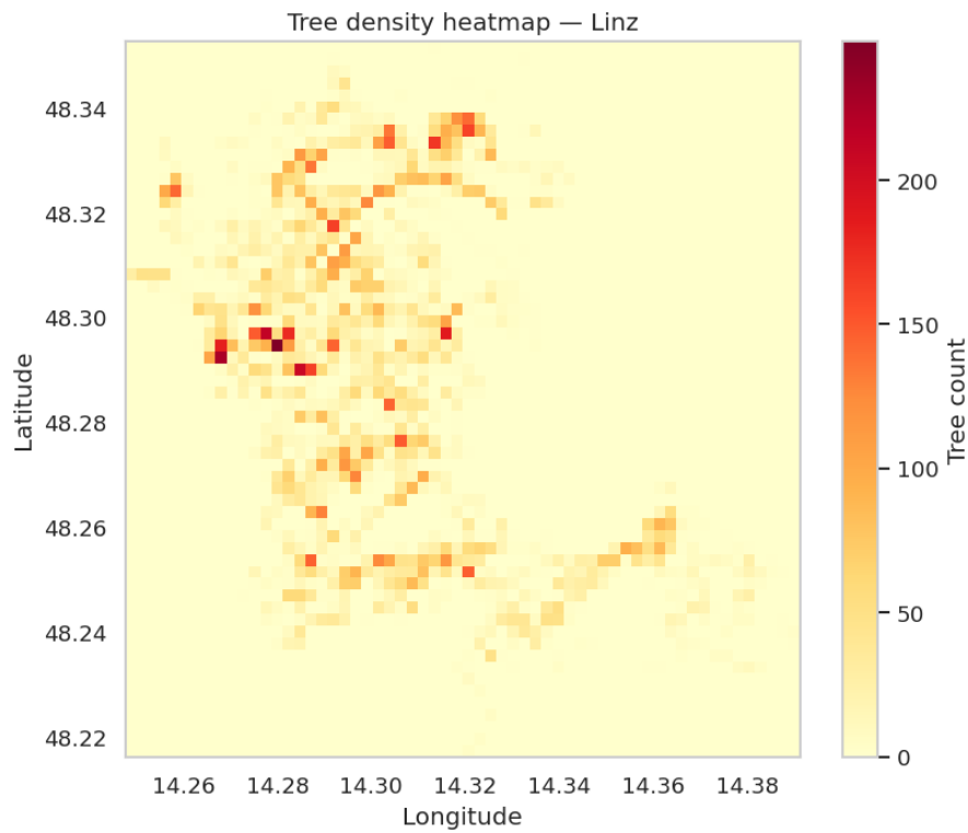
Figure 25: Tree density heatmap. Linz.
