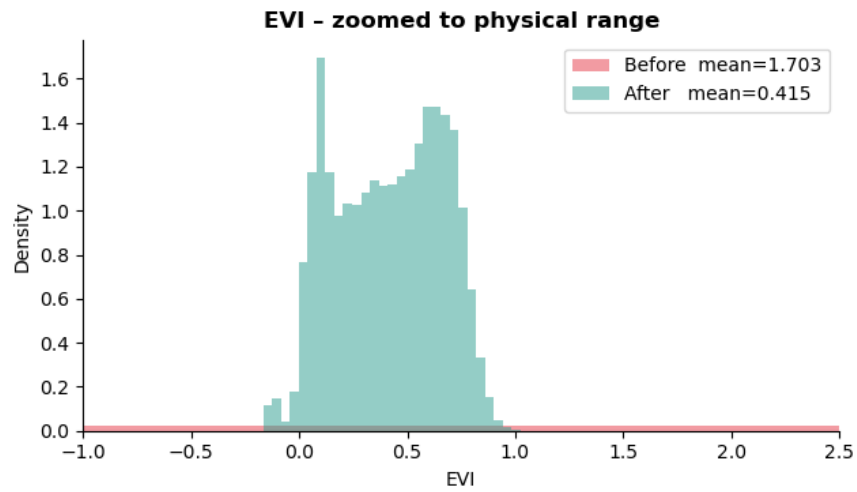
Figure 13: EVI — zoomed to the physical range.
