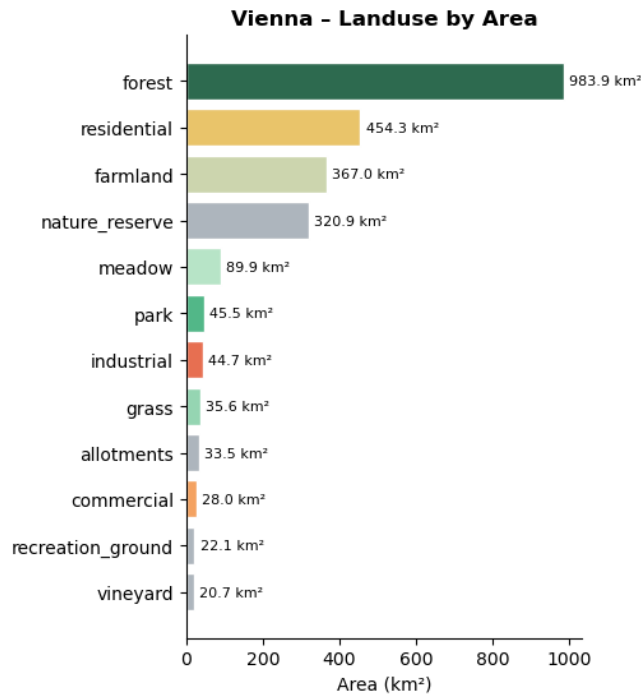
Figure 18: Land use distribution by area per city. Vienna.
