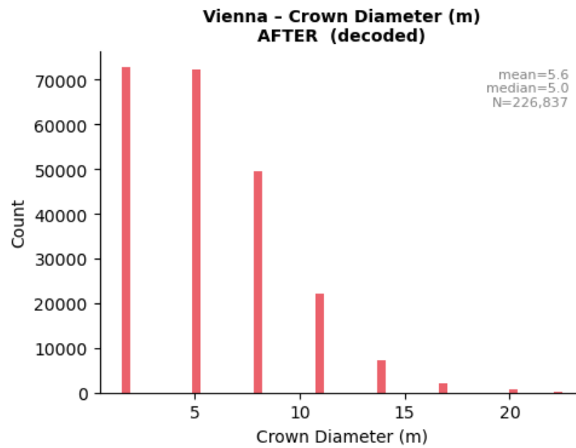
Figure 7: Vienna — crown diameter, after correction (decoded to metres).
