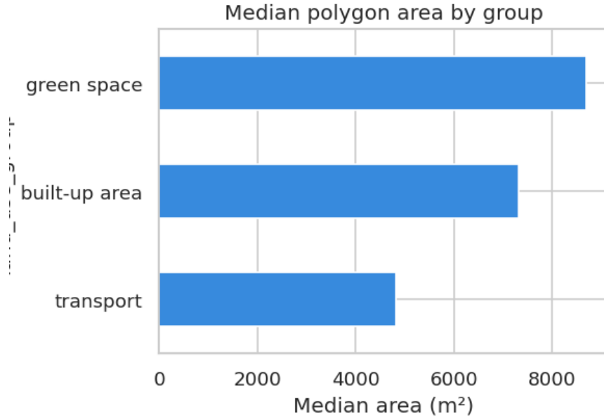
Figure 28: Median polygon area by group.
