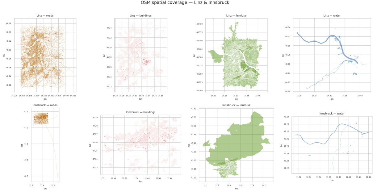
Figure 27: Spatial coverage Linz and Innsbruck.
