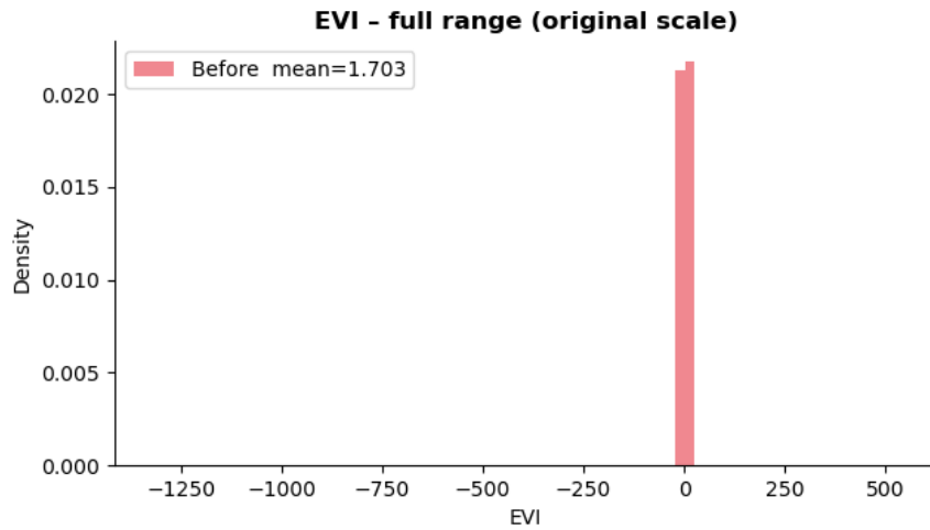
Figure 11: EVI — full range (original scale).
