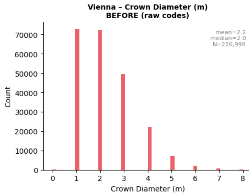
Figure 5: Vienna — crown diameter, before correction (raw codes).
