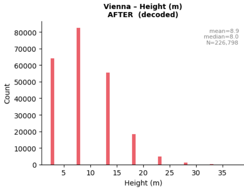
Figure 6: Vienna — tree height, after correction (decoded to metres).
