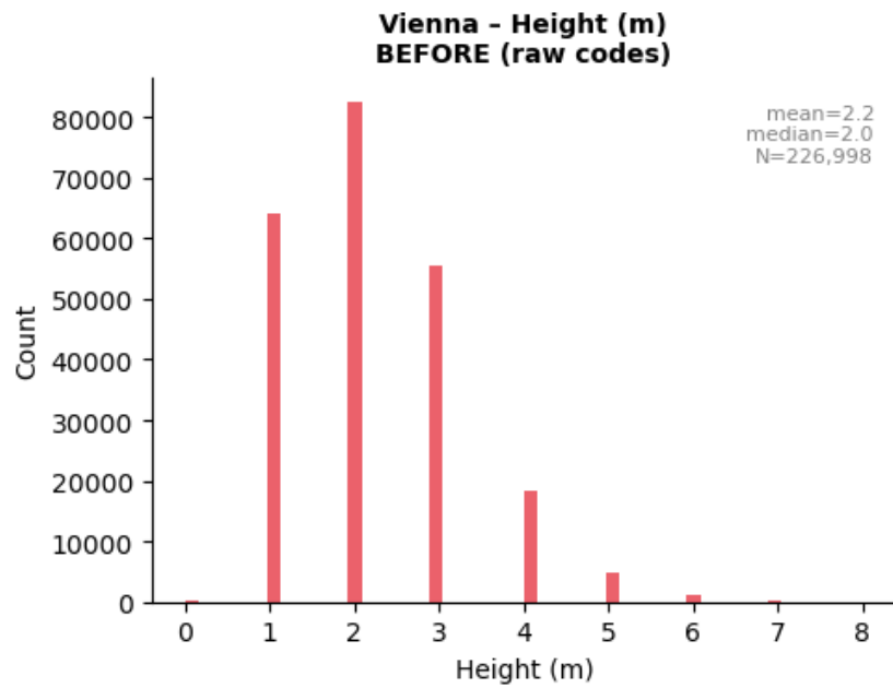
Figure 4: Vienna — tree height, before correction (raw ordinal codes).
