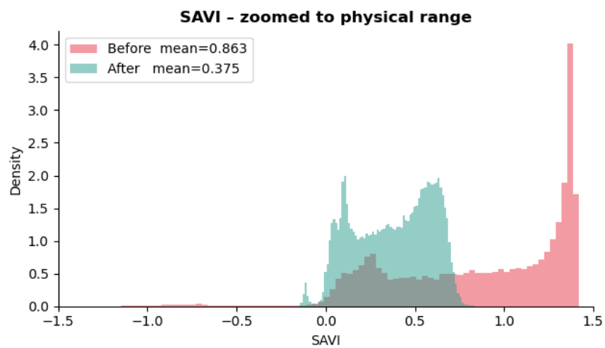
Figure 14: SAVI — zoomed to the physical range.
