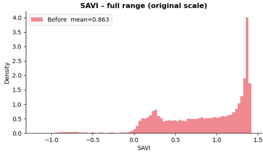
Figure 12: SAVI — full range (original scale).
